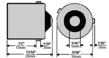
BAU15s Bayonet Single Conductor
